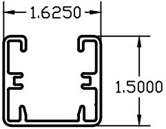
SIDE RAIL PROFILE
